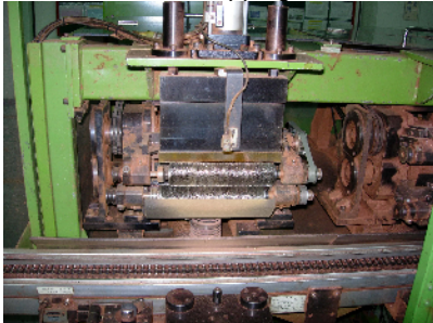
Enameled Wire Stripping Device
